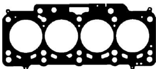
726.740 1 ⊗ | ± 1,55 mm
